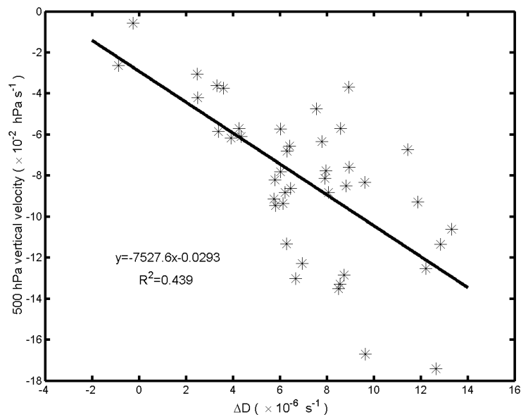
Figure 5.23: The relationship between 500 hPa vertical velocity and \Delta D (the difference between the divergence at 200 hPa and 850 hPa). The linear least-squares regression line is statistically significant.
