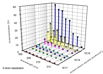
Fig. 3.2 – Magnitude of underestimation in standard DOAS measurements conducted at 0.4 nm optical resolution caused by a non-commutative cross-section convolution. Errors are slightly smaller than for 0.8 nm optical resolution (Fig. 3.1) and again occur for high column densities S and short wavelengths \lambda .
