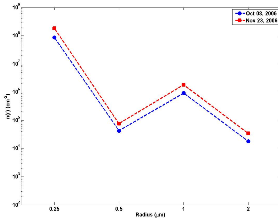
Fig. 1. Aerosol size distribution for Oct 8, 2006 and Nov 23, 2006 with \alpha = 1.01 , \text{AOD}_{440 \text{ nm}} = 0.15 and 0.31 , respectively.
