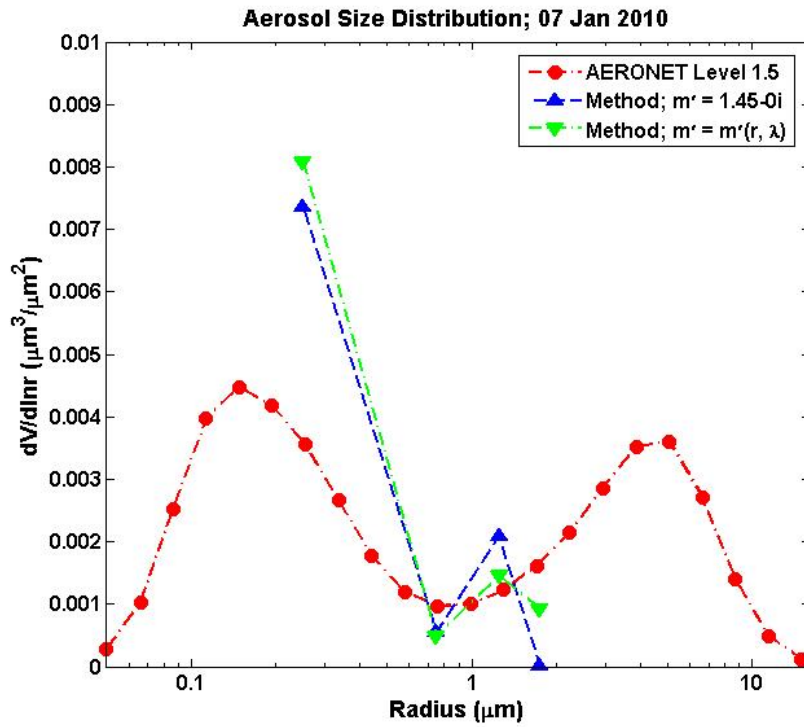
Fig. 2. Daily-averaged aerosol size distribution ( \text{micron}^3 / \text{micron}^2 ) for 7 January 2010 for Zanjan, Iran. AERONET and our method with old and new refractive indices are employed respectively.
