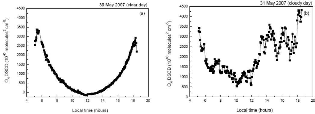
Fig. 7. Diurnal variations of the O 4 DSCDs on a clear (30 May 2007, a) and a cloudy day (31 May 2007, b), respectively.
