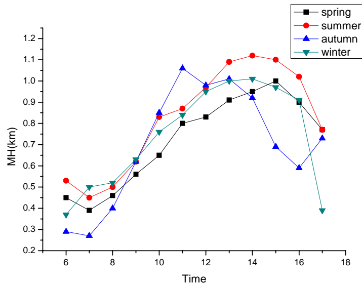
Figure, The diurnal variation of MH in different season
